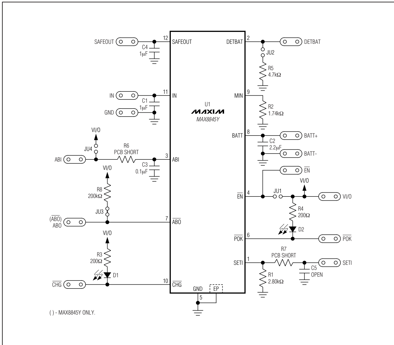
Figure 3. MAX8845Y EV Kit Schematic
