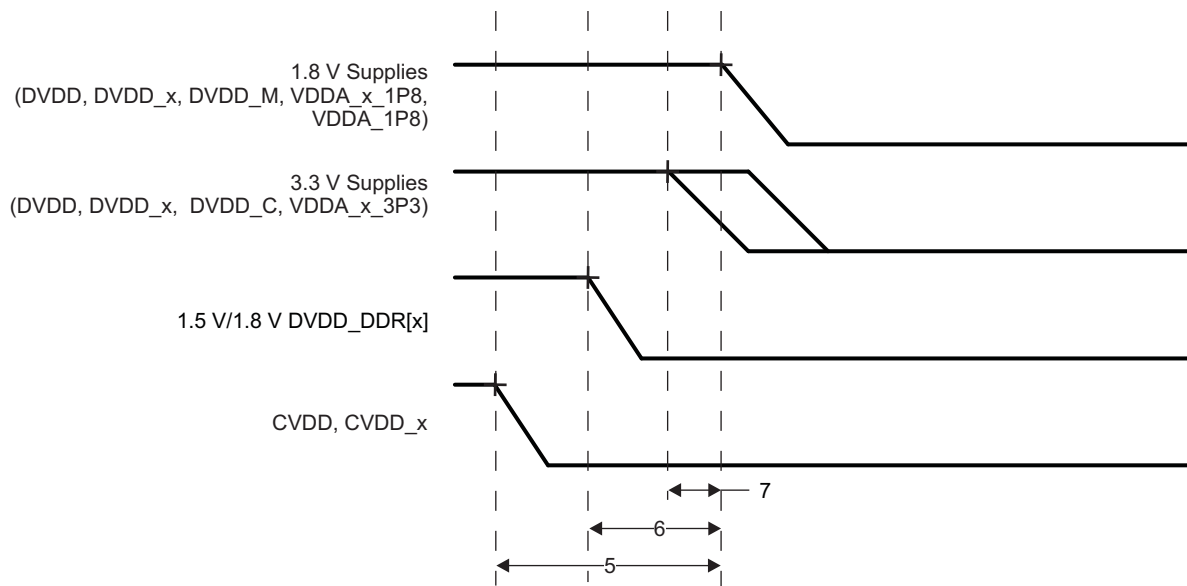
Figure 7-3. Power-Down Sequence
