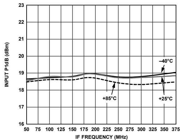
Figure 47. Input P1dB vs. IF Frequency
