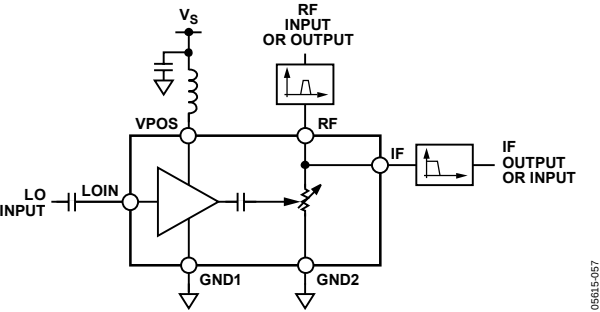
Figure 57. Simplified Schematic
