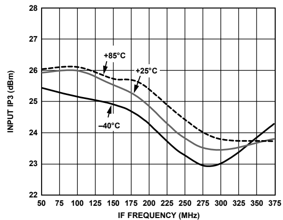
Figure 46. Input IP3 vs. IF Frequency
