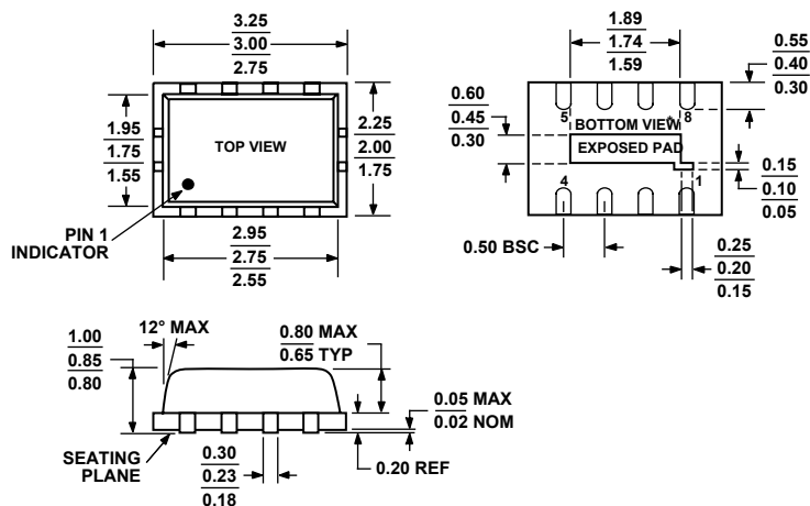
Figure 66. 8-Lead Lead Frame Chip Scale Package [LFCSP_VD] 2 mm x 3 mm Body, Very Thin, Dual Lead (CP-8-1) Dimensions shown in millimeters
