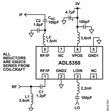
Figure 63. 3.3 GHz to 3.8 GHz RF Downconversion Schematic
