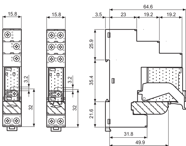
4C.01 / 4C.02 Screw terminal
