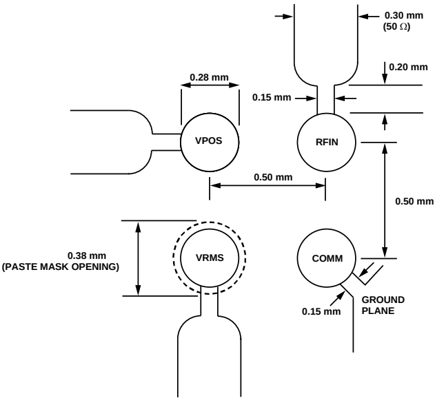
Figure 47. Land Pattern Used on the ADL5500 Evaluation Board
