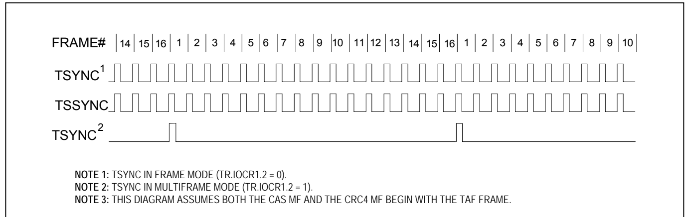
Figure 12-25. Transmit-Side Timing
