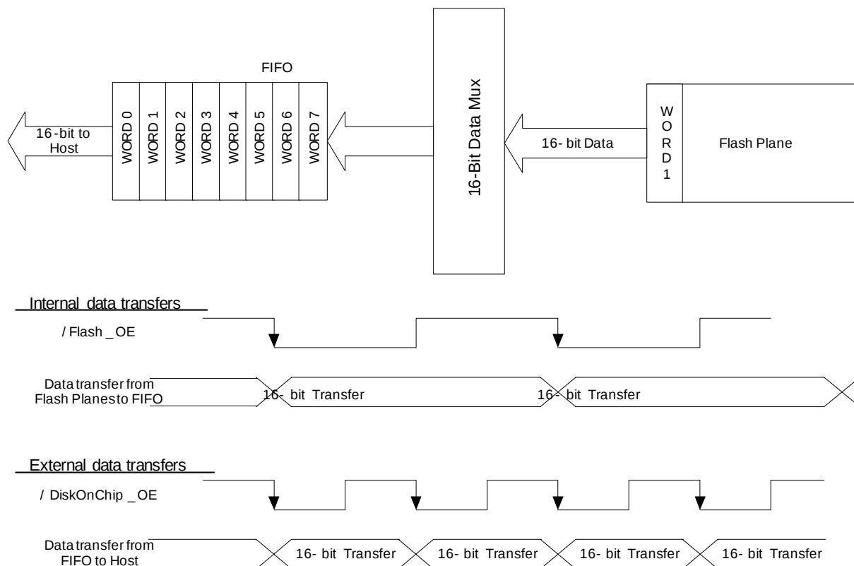
Figure 8: MultiBurst Operation
