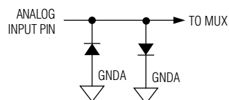
ANALOG INPUT EQUIVALENT CIRCUIT TYPE 6: ADC INPUT
