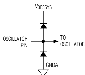
OSCILLATOR EQUIVALENT CIRCUIT TYPE 8: OSCILLATOR I/O
