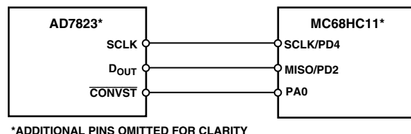
Figure 18. Interfacing to the MC68HC11
