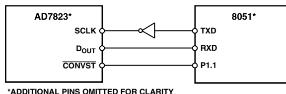
Figure 19. Interfacing to the 8051 Serial Port
