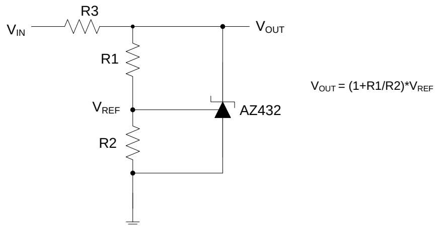
Shunt Regulator
