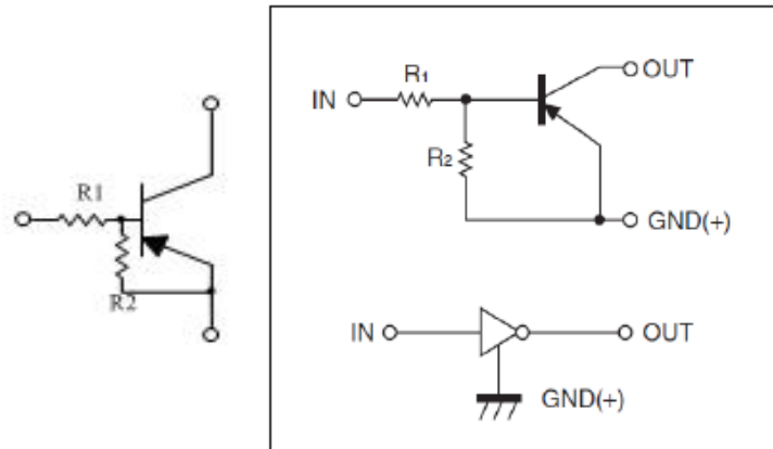
Equivalent Circuit
