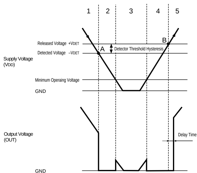
FIG. 2 Operation Diagram
