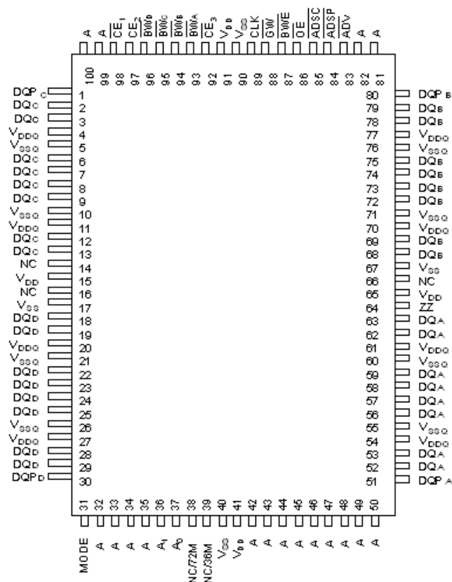
CY7C1380DV33 (512 K × 36)
