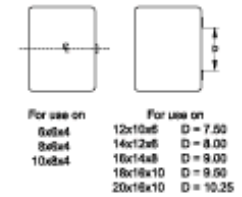
Latch Locations
