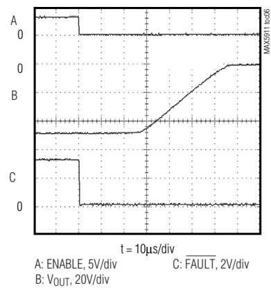
MAX5911 ZERO-CURRENT RESPONSE
