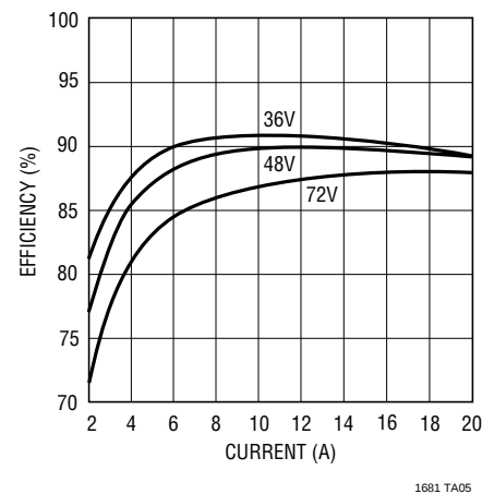
LT1681/LTC1698 Isolated 3.3V/20A Converter Efficiency vs Load Current
