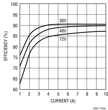
LT1681/LTC1698 Isolated 5V/10A Converter Efficiency vs Load Current
