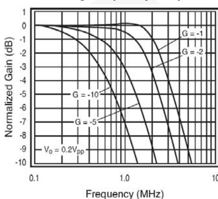
Figure 8. Inverting Frequency Response
