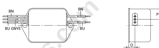
Connection style -07, 16A types (same dimensions as style -06)
