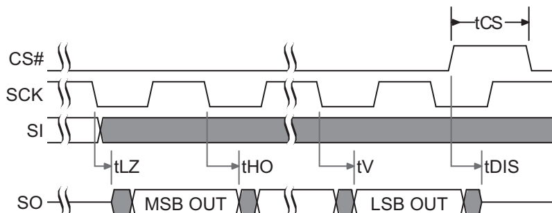
Figure 6.11 SPI SDR MIO Timing
