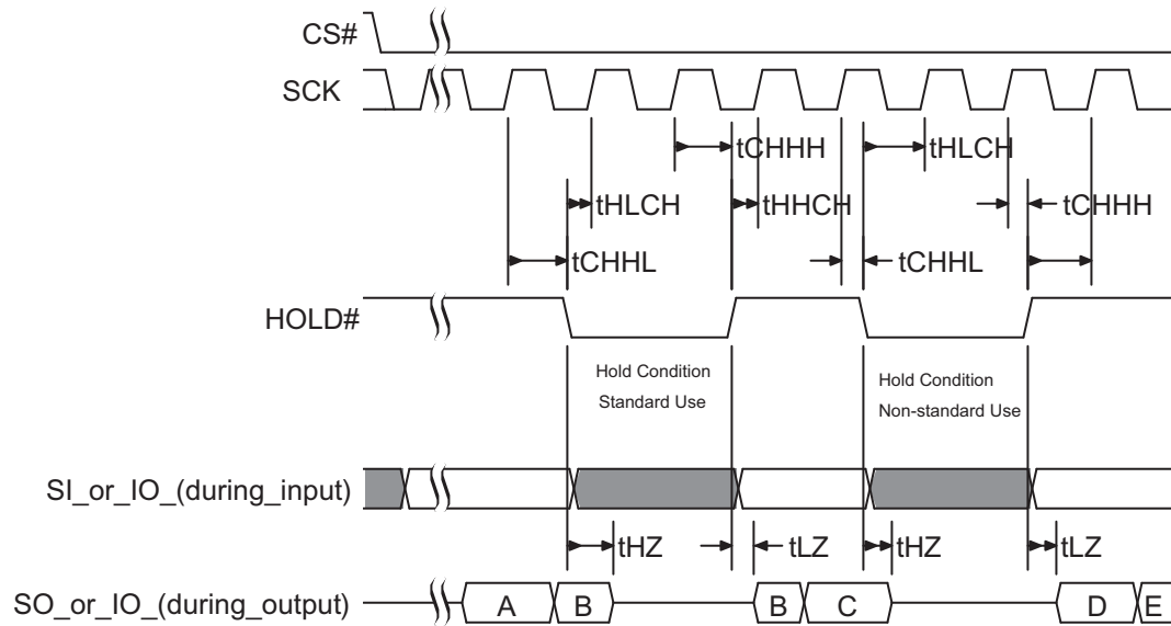
Figure 6.12 Hold Timing
