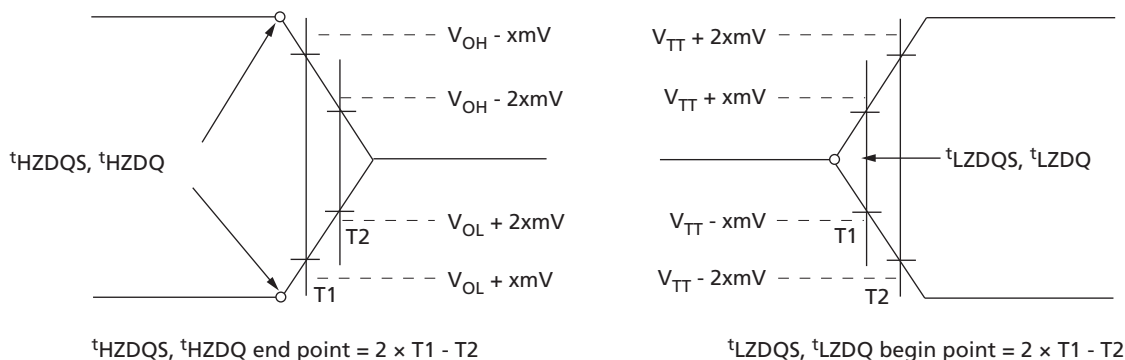
Figure 80: Method for Calculating t_{HZ} and t_{LZ}
