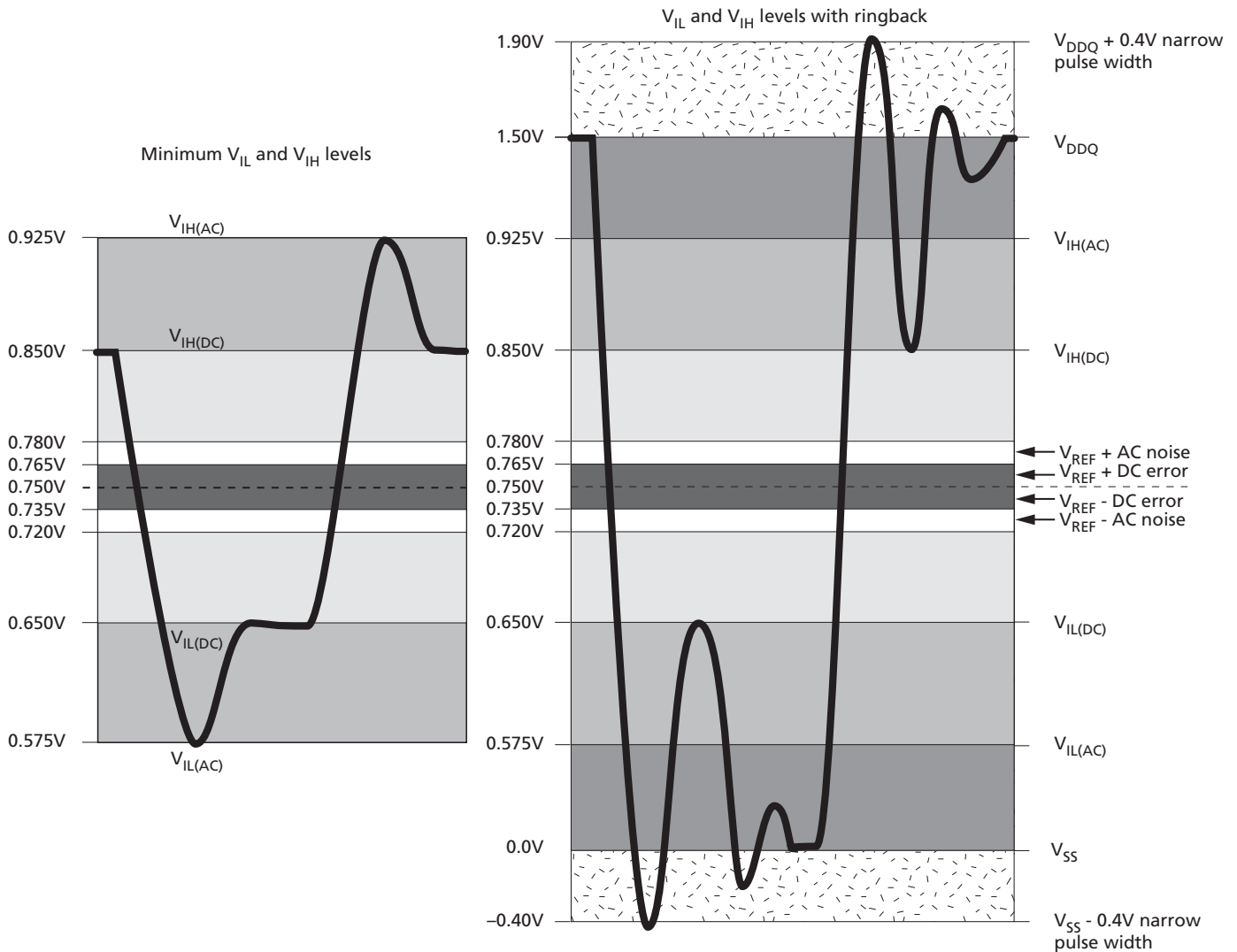
Figure 15: Input Signal
