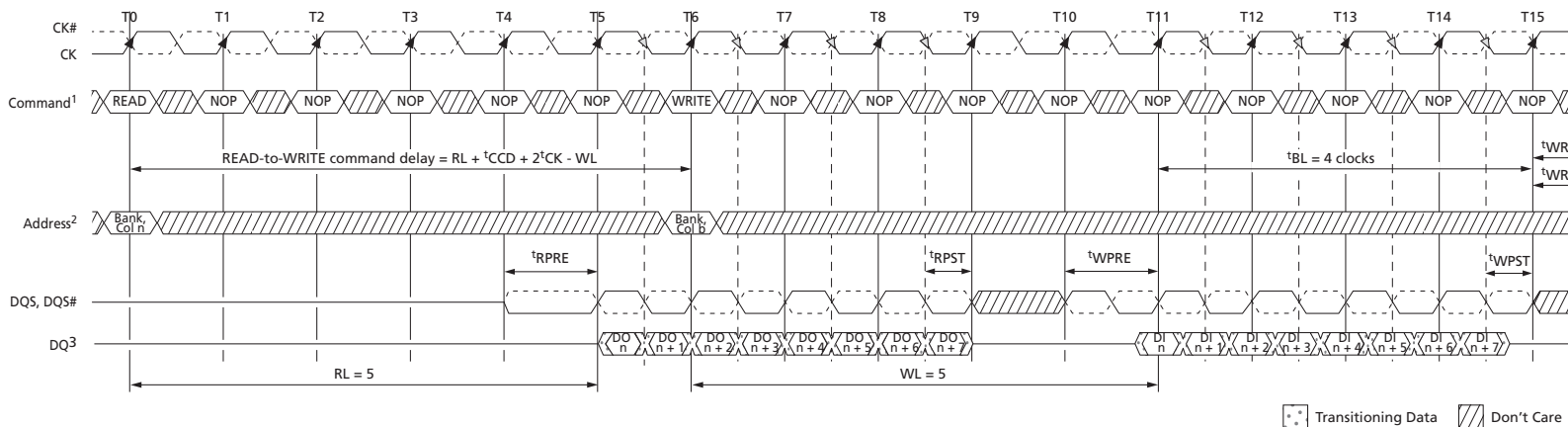
Figure 72: READ (BL8) to WRITE (BL8)
