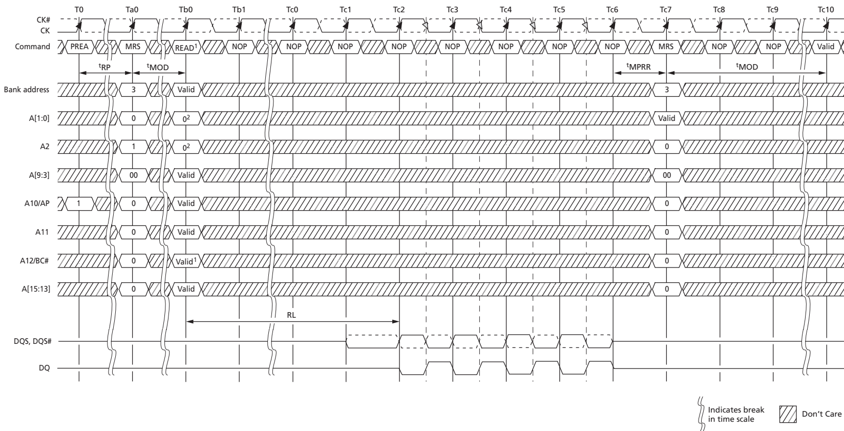
Figure 61: MPR System Read Calibration with BL8: Fixed Burst Order Single Readout
