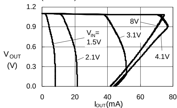
S-817A11A(Ta=25°C)
