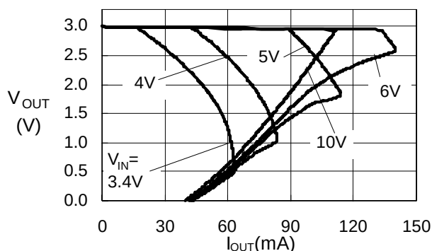
S-817B11A(Ta=25°C)
