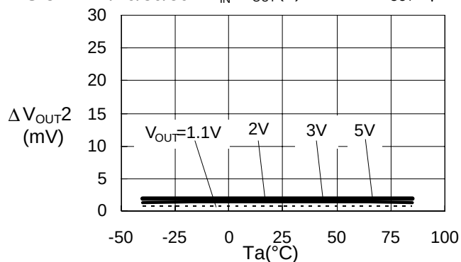
(7) LINE REGULATION 2 versus AMBIENT TEMPERATURE
