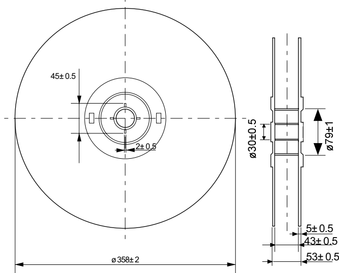
No. YF003-A-R-SD-2.0
