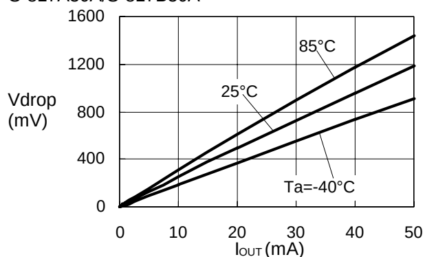
S-817A30A/S-817B30A
