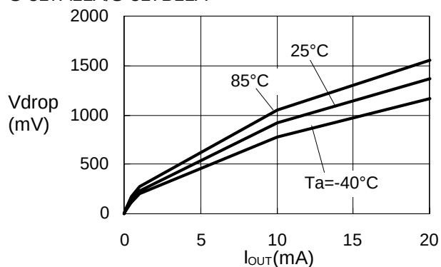
S-817A11A/S-817B11A
