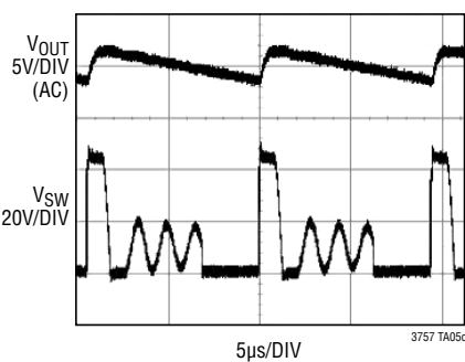
Switching Waveforms
