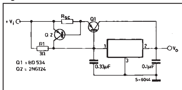
Figure 7 : Short-circuit Protection.
