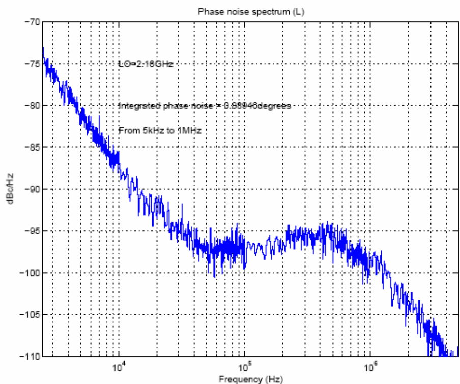
Figure 6. Phase Noise Performance for Si2107/08/09/10 (Typical)
