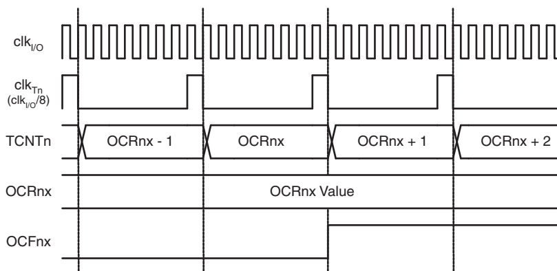
Figure 4-55. Timer/Counter Timing Diagram, Setting of OCF1A/B, with Prescaler ( f_{clk\_I/O}/8 )
