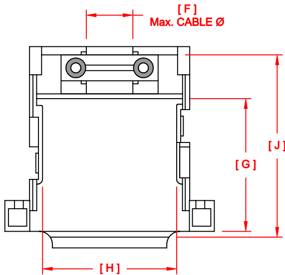
INTERNAL VIEW WITH YOKE INSERTED
