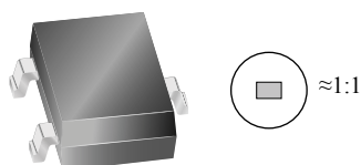
Package LH, 3-pin SOT
