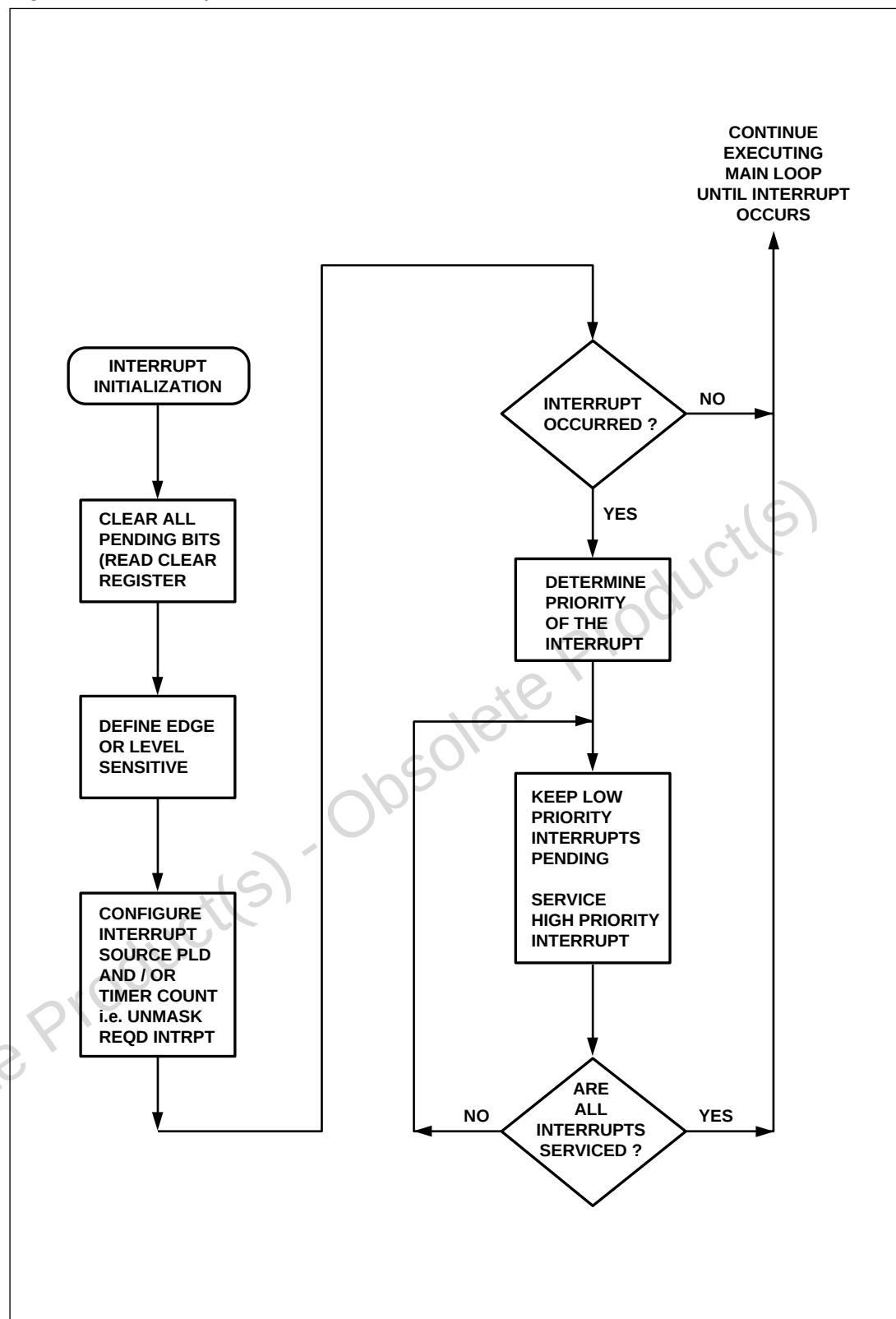
Figure 48. Interrupt Flowchart
