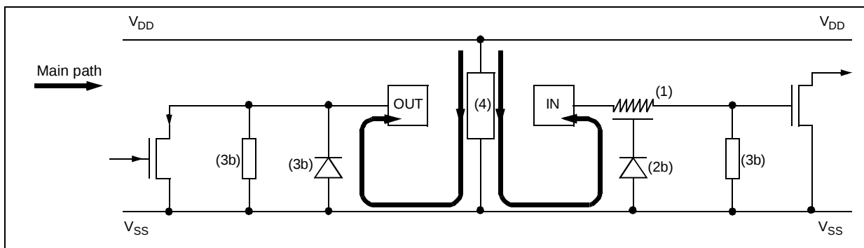
Figure 81. Multisupply Configuration
