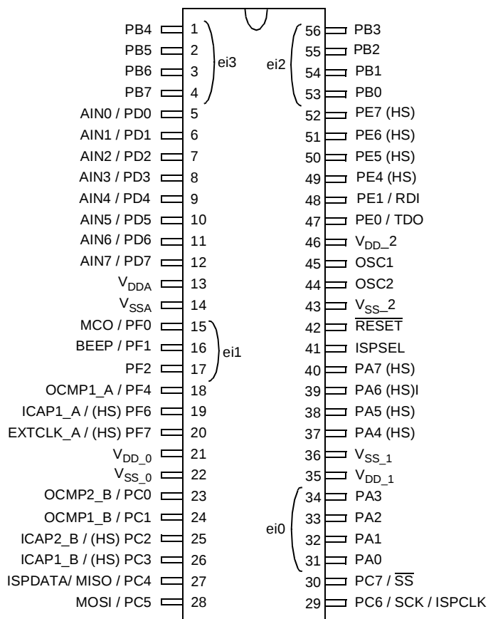
Figure 3. 56-Pin SDIP Package Pinout (N versions)
