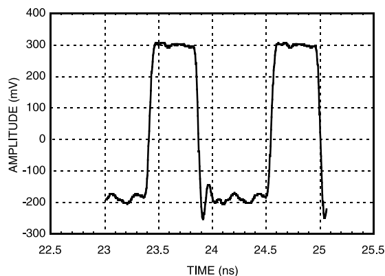
Output Voltage Waveform, P_{in} = 0\text{ dBm} , F_{out} = 882\text{ MHz} , T = 25\text{ }^{\circ}\text{C}
