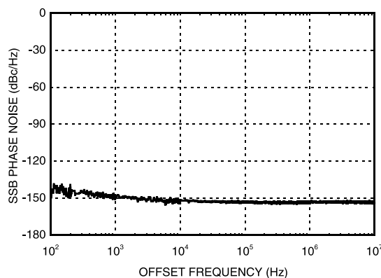
SSB Phase Noise Performance, P_{in} = 0\text{ dBm} , F_{in} = 6\text{ GHz} , T = 25^\circ\text{C}
