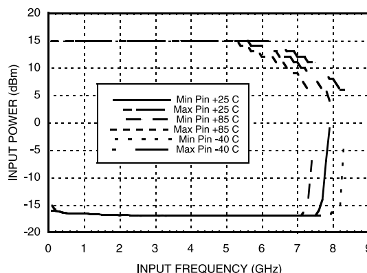
Input Sensitivity Window vs. Temperature
