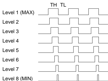
(a) BZ signal
