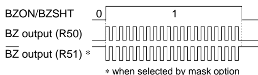
Fig. 5.6.5.14 BZ ( \overline{\text{BZ}} ) output waveform
