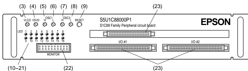
Fig. B.1.2 Panel layout (S5U1C88000P1)
