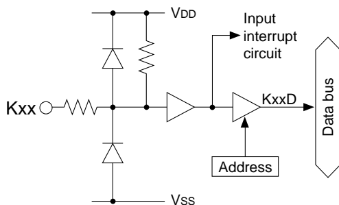
Fig. 5.5.1.1 Structure of input port
