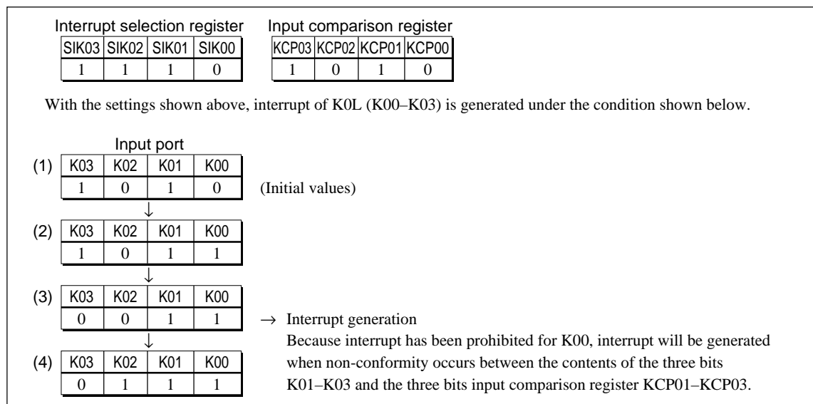
Fig. 5.5.3.2 Interrupt generation example in K0L (K00–K03)
