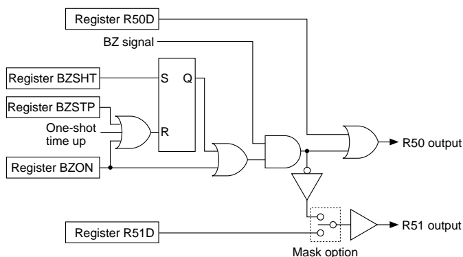
Fig. 5.13.2.1 Configuration of R50 and R51
