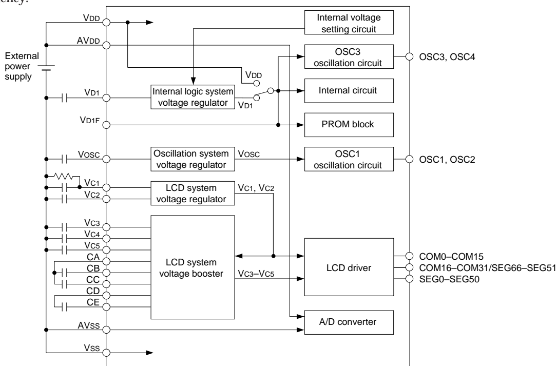
Fig. 2.2.1 Configuration of power supply circuit
