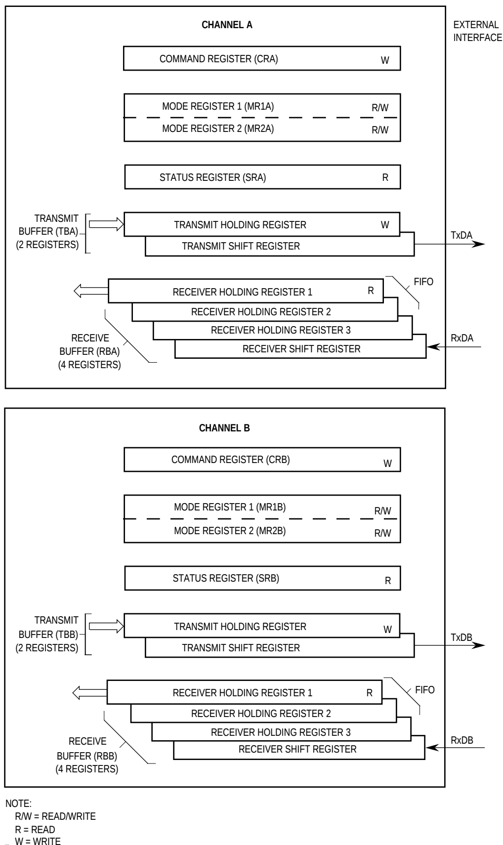
Figure 6-4. Transmitter and Receiver Functional Diagram
