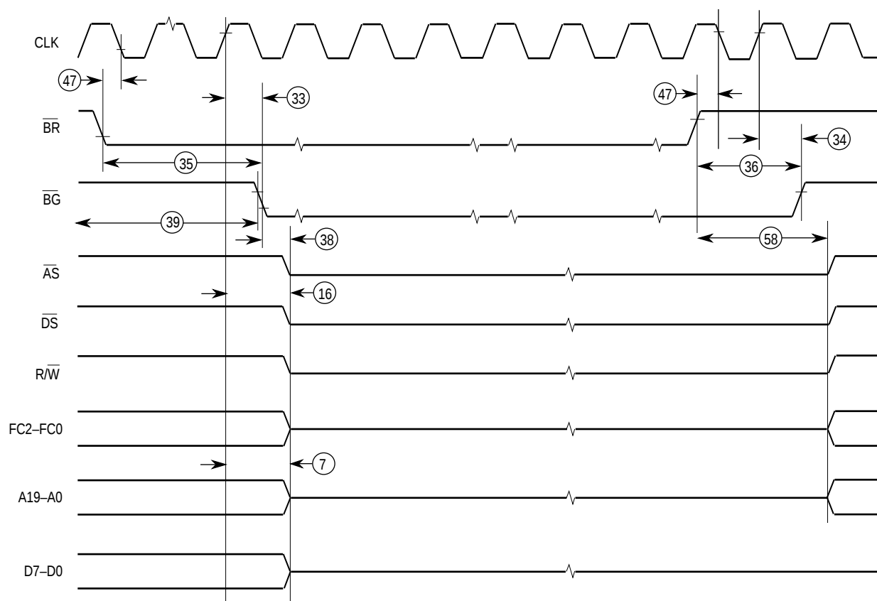
Figure 8-6. Bus Arbitration Timing Diagram
