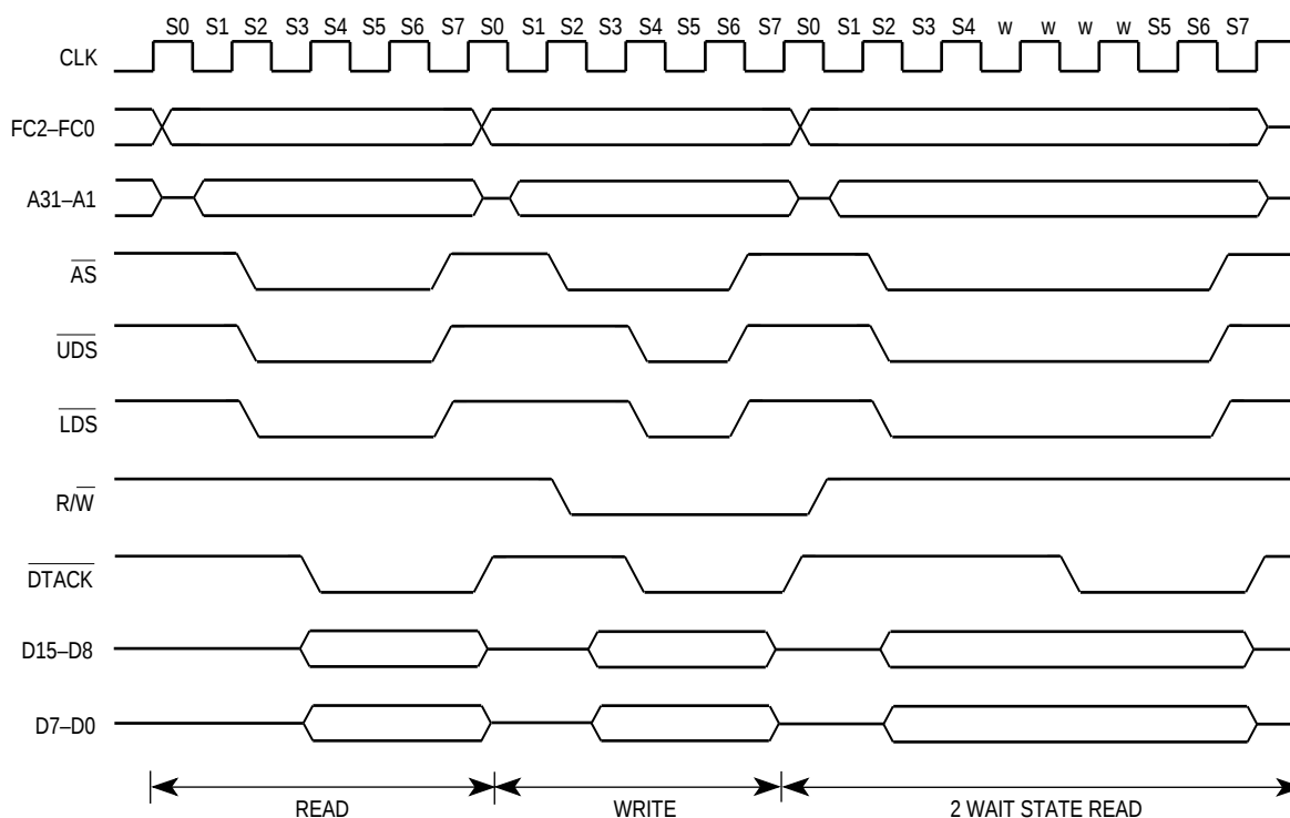
Figure 3-3. Read and Write Cycle Timing Diagram
