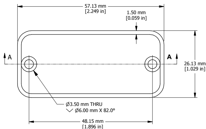
CLOSED BEZEL
