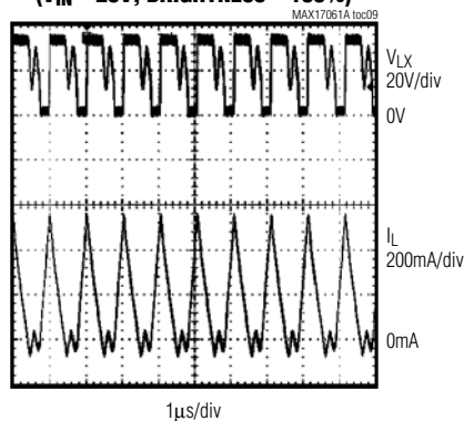
SWITCHING WAVEFORMS ( V_{IN} = 20V , BRIGHTNESS = 100%)
