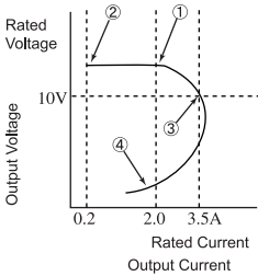
Fig2. Output Voltage/Current
