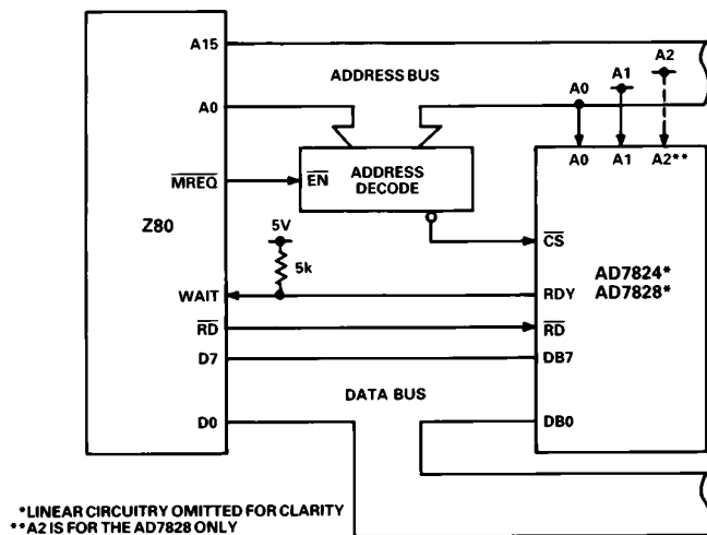
Figure 16. AD7824/AD7828–Z80 Interface
