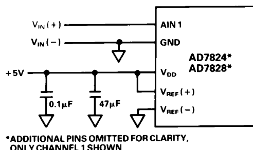
Figure 5. Power Supply as Reference
