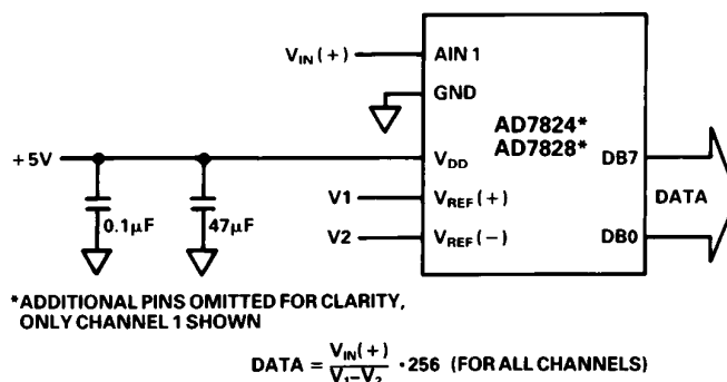
Figure 7. Input Not Referenced to GND
