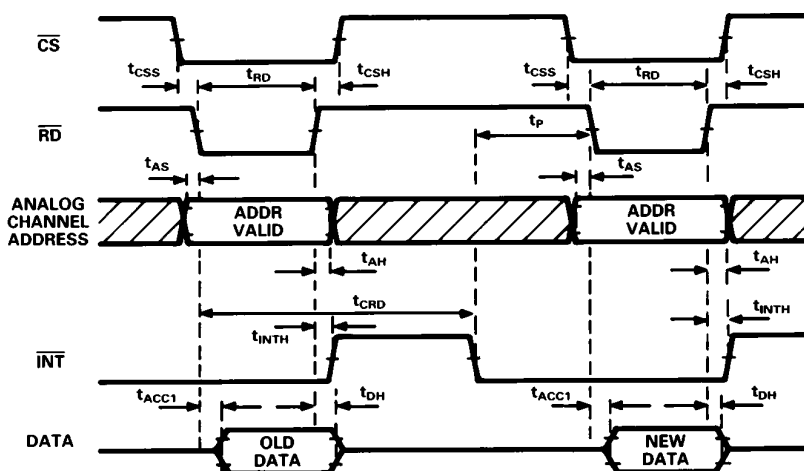
Figure 15. Mode 1 Timing Diagram
