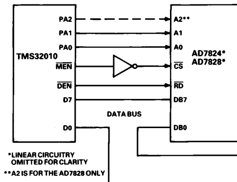
Figure 18. AD7824/AD7828–TMS32010 Interface
