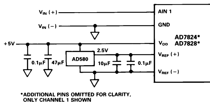
Figure 6. External Reference Using the AD580, Full-Scale Input is 2.5 V
