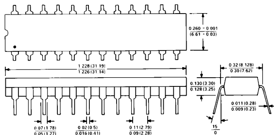
24-Pin Plastic DIP (N-24)
