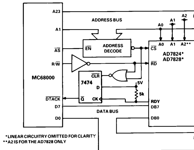
Figure 17. AD7824/AD7828–MC68000 Interface
