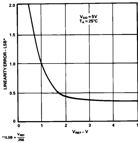
Accuracy vs. V_{\text{REF}} [ V_{\text{REF}} = V_{\text{REF}}(+)-V_{\text{REF}}(-) ]
