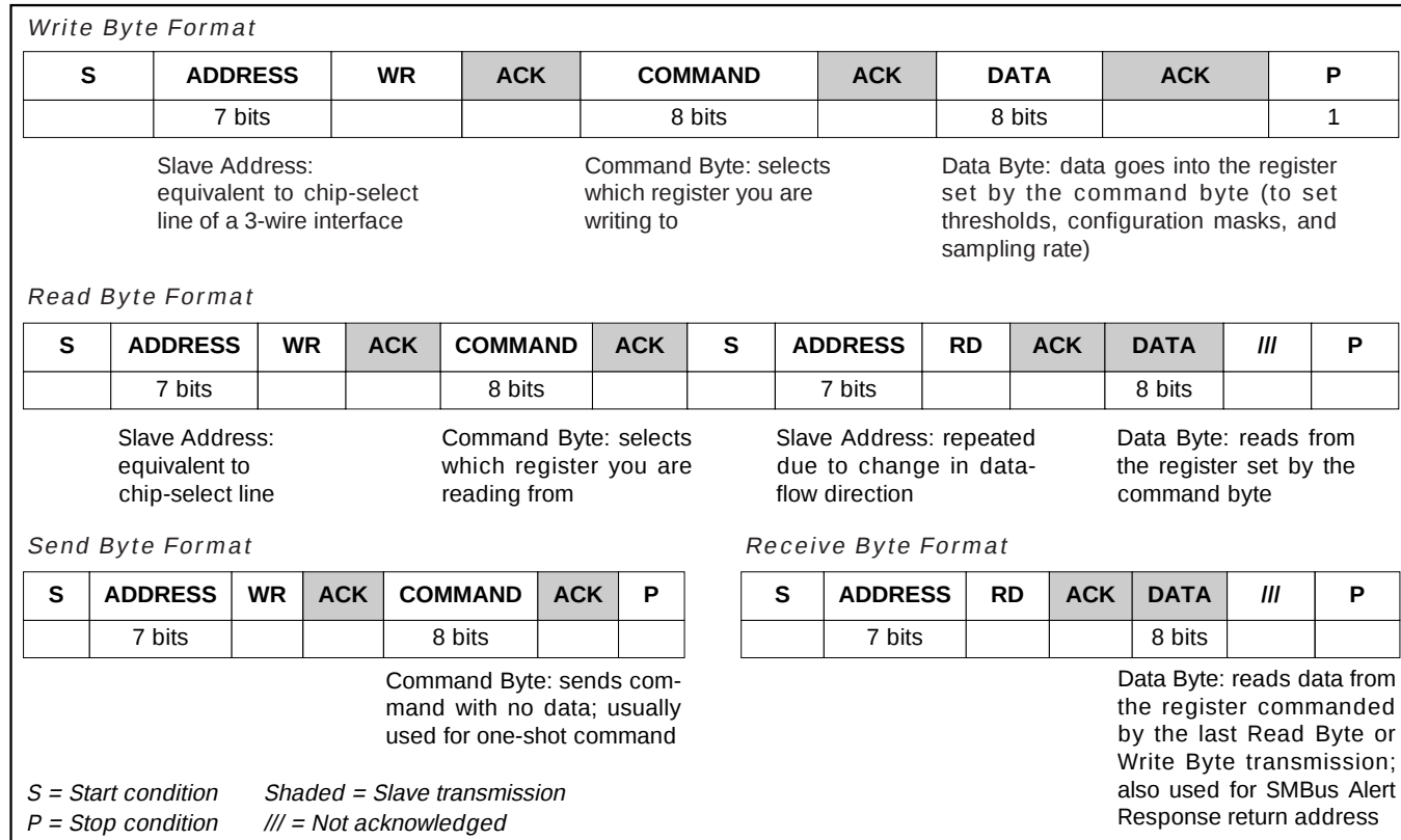
Figure 3. SMBus Protocols
