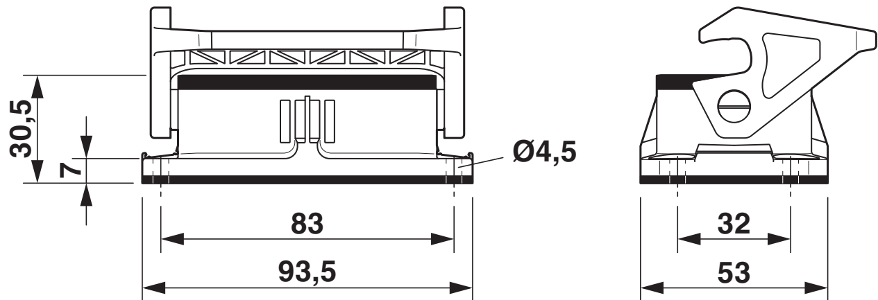
Dimensioned drawing
