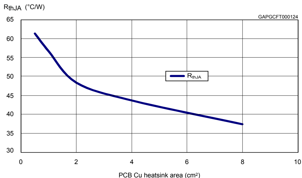
Figure 28. R_{thJA} vs PCB copper area in open box free air condition (one channel ON)
