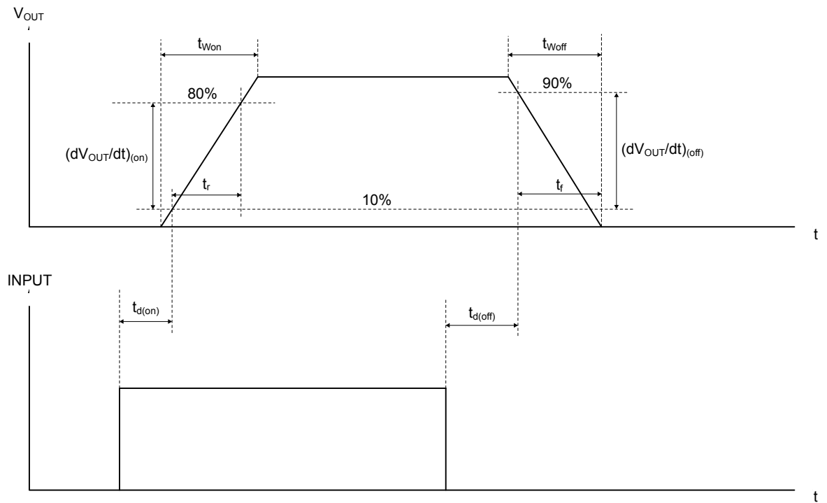
Figure 9. Switching characteristics
