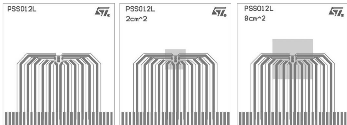
Figure 27. PowerSSO-12 PCB
