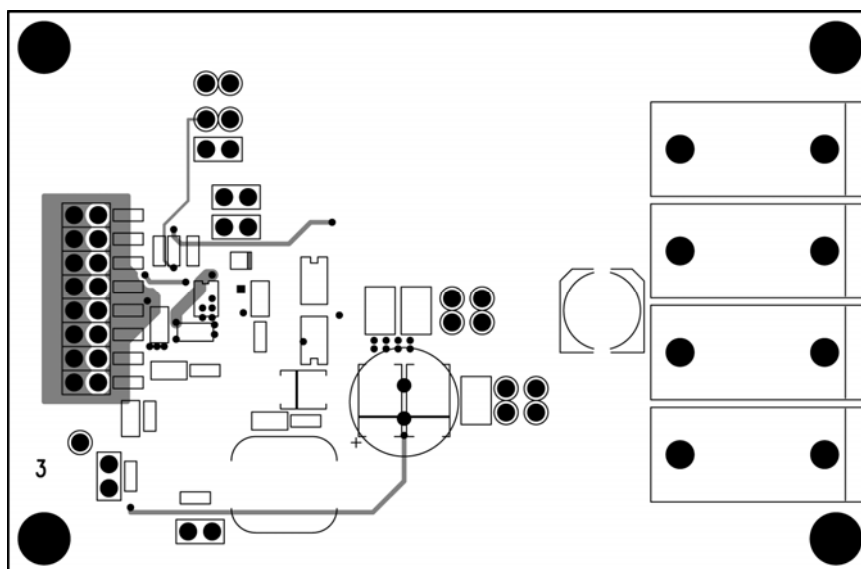
Figure 15. MIC2165 10A Evaluation Board Mid-Layer 2
