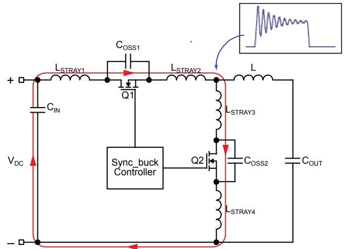
Figure 6. Output Parasitics
