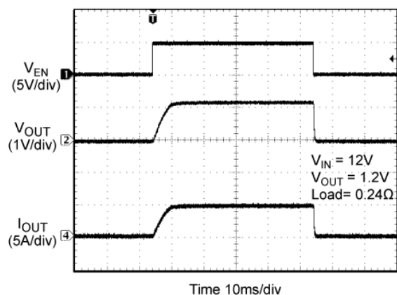
Power-Up/Power-Down
