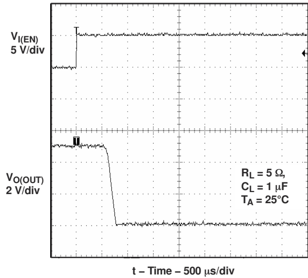
Figure 6-31. Turnoff Delay and Fall Time With 1-μF Load
