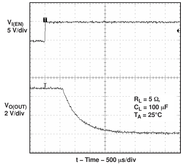
Figure 6-33. Turnoff Delay and Fall Time With 100-μF Load
