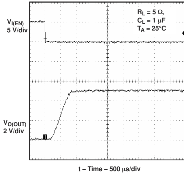
Figure 6-30. Turnon Delay and Rise Time With 1-μF Load
