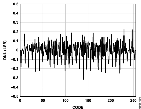
Figure 30. DNL, f_{IN} = 2.4 MHz, f_{SAMPLE} = 100 MSPS
