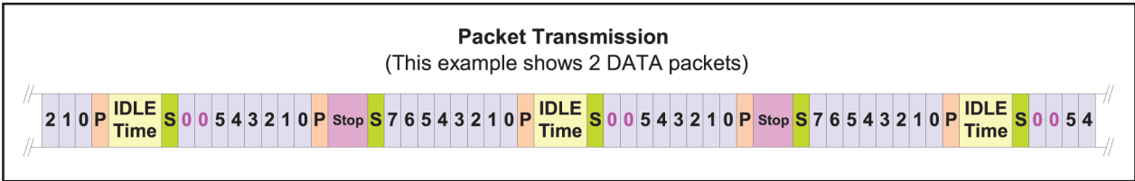
Figure 17: Transmission of data packets (NPA-600 pressure only mode)
