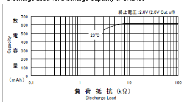
Discharge Load vs. Discharge Capacity of CR2450
