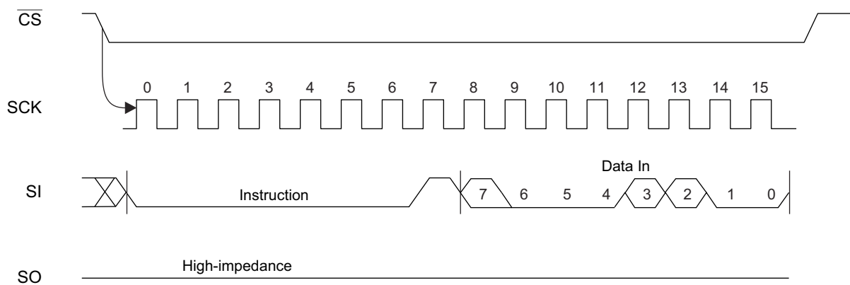
Figure 6-5. WRSR Timing
