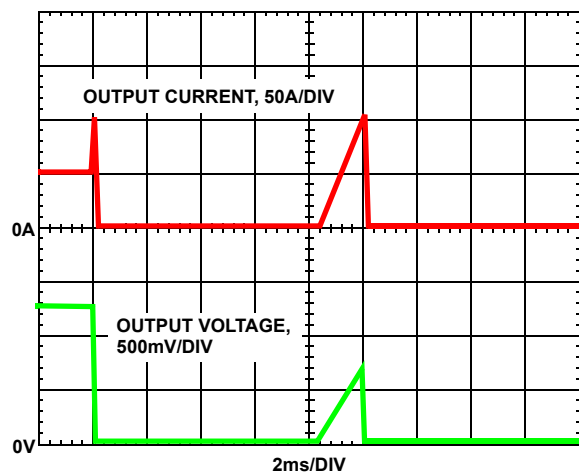
FIGURE 14. OVERCURRENT BEHAVIOR IN HICCUP MODE F_{SW} = 500kHz
