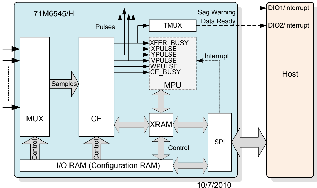
Figure 22: Data Flow
