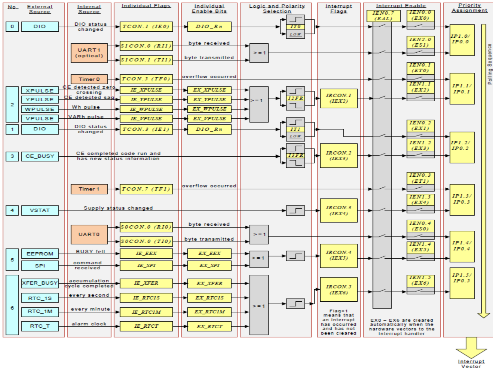
Figure 12: Interrupt Structure
