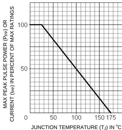
FIGURE 2 PULSE DERATING CURVE (prior to impulse)
