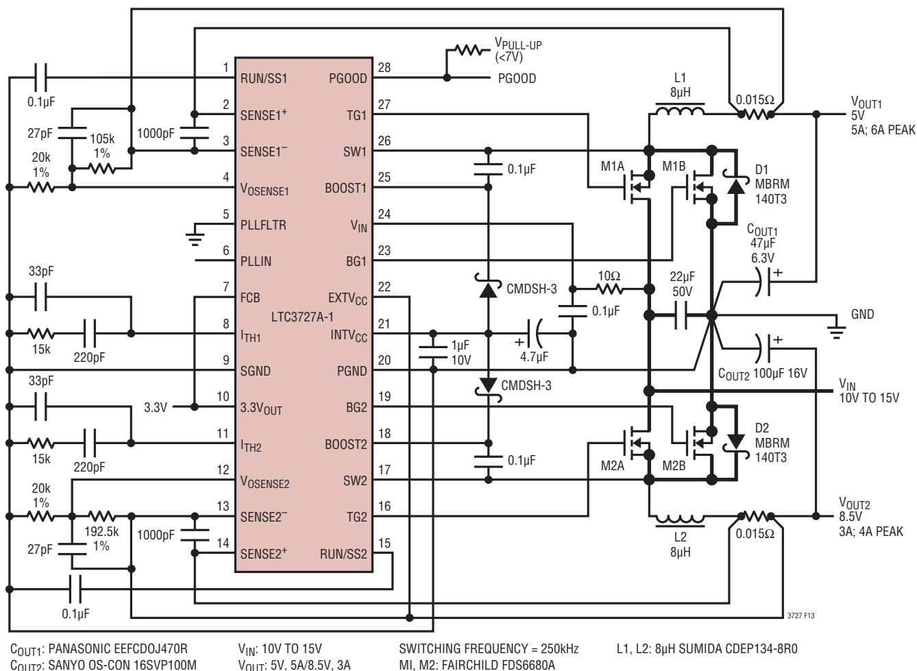
Figure 13. LTC3727A-1 8.5V/3A, 5V/5A Regulator
