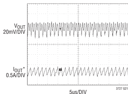
Constant Frequency (Burst Inhibit) Operation (Figure 13)
