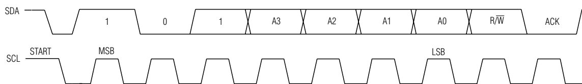
Figure 6. Slave Address
